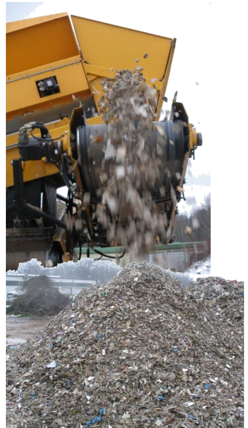
Excavator-loading into the 3-fraction starscreen 3-mtb
